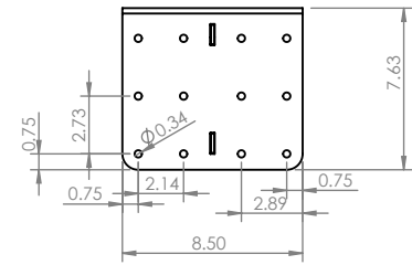
Sleeve Detail
